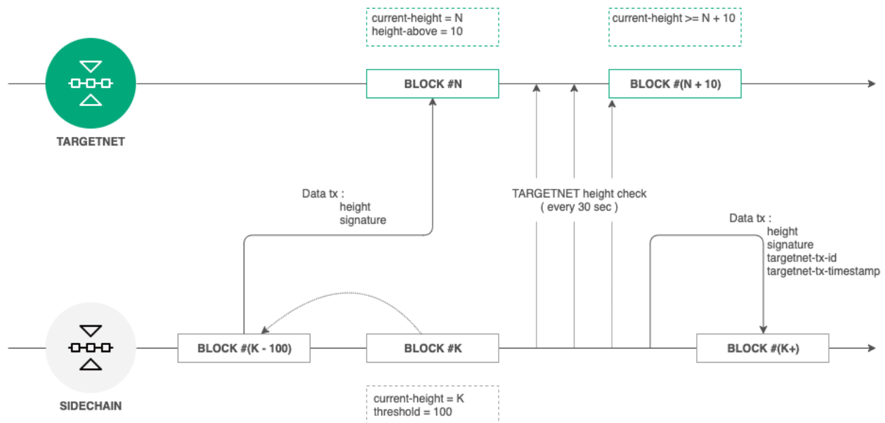
Fig. 1: Targetnet anchoring scheme
